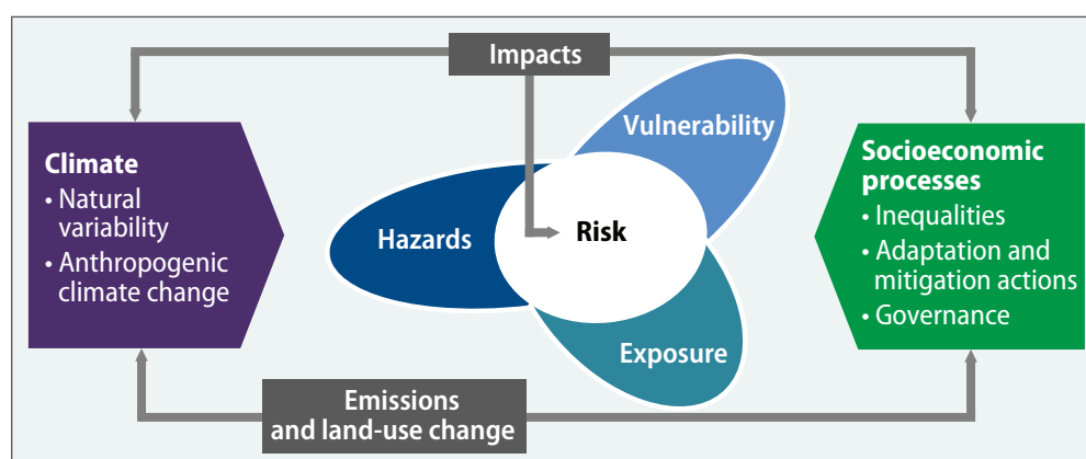
Figure V.5 Human interface with the climate
